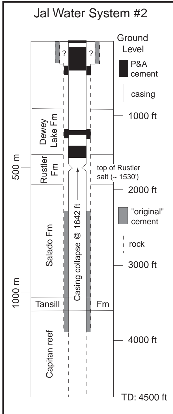
Figure 5. General stratigraphy and casing and cementing record for Skelly Jal Water System #2, located adjacent to the WRS.
